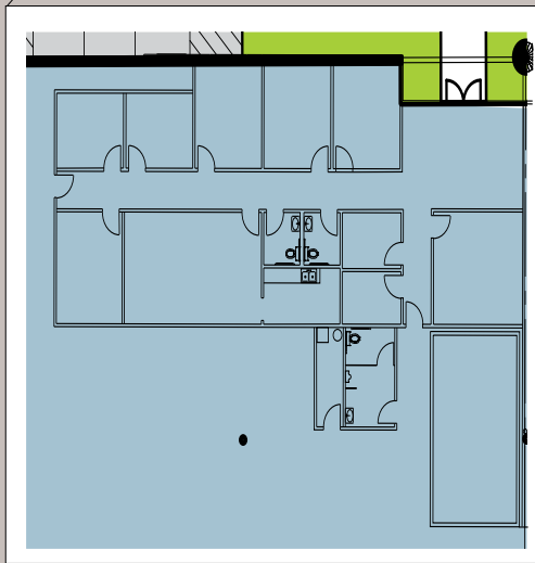
OFFICE LAYOUT
