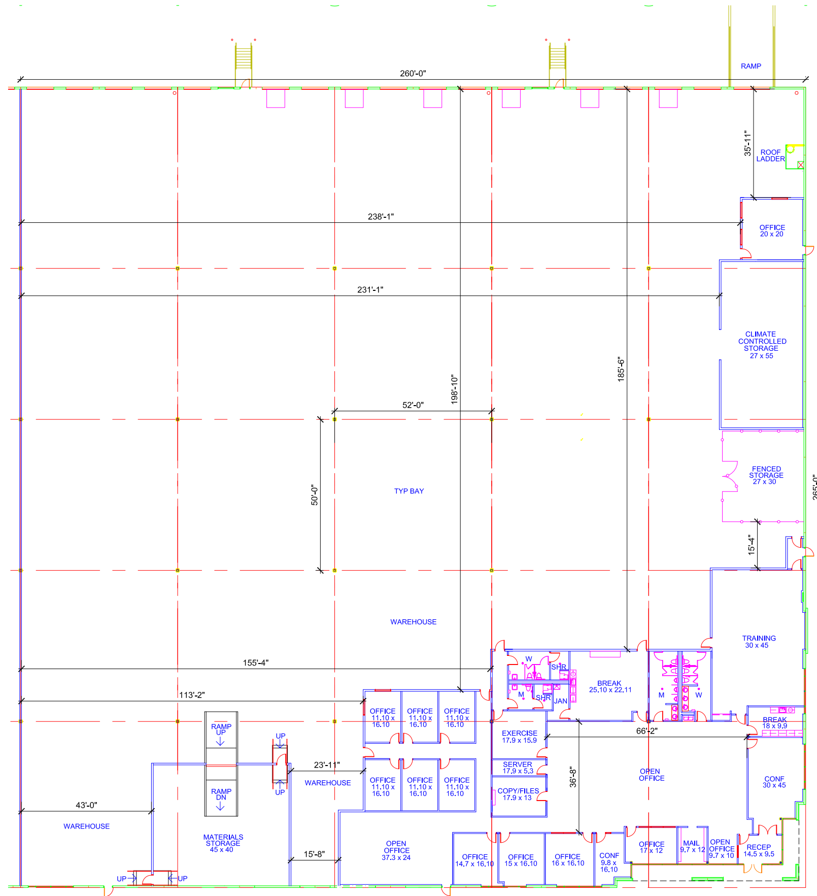
FLOOR PLAN
